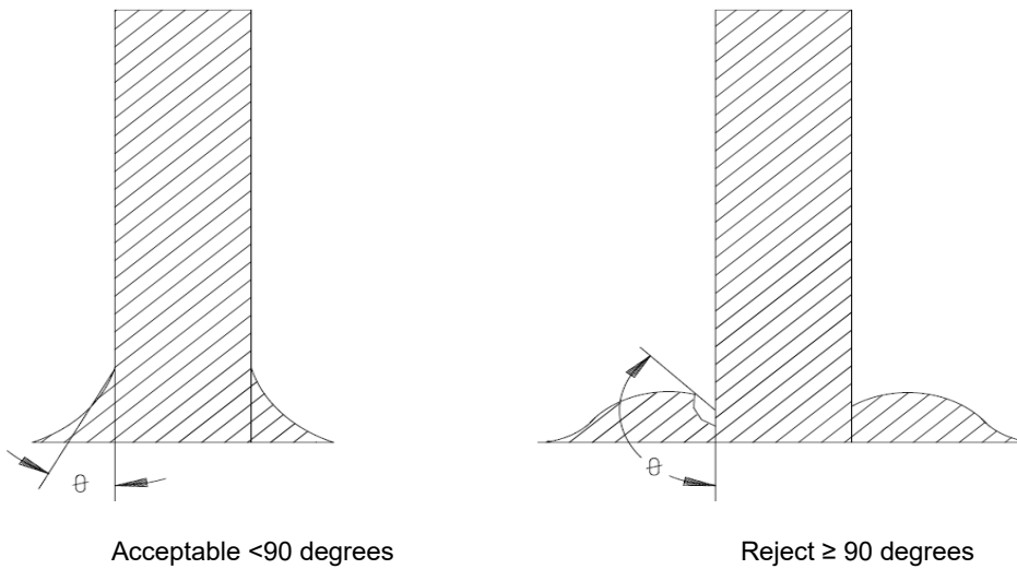
FIGURE 2003-11. Acceptable wetting angle for column grid arrays.
