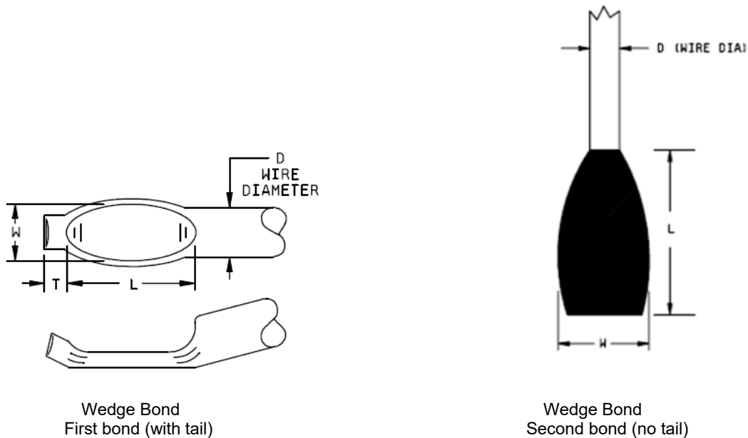
Figure 2017-16a. Bond Dimensions .
