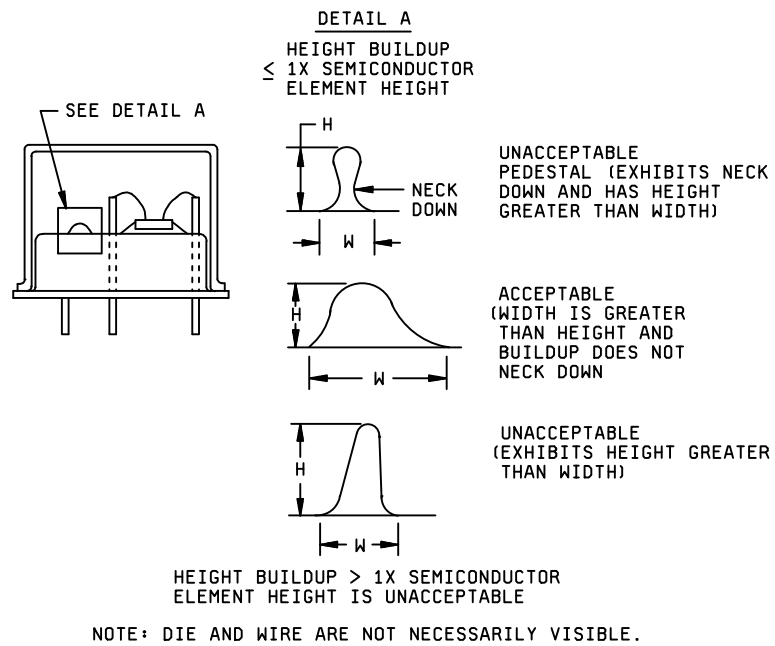
FIGURE 2012-4. Extraneous bonding material build-up.
