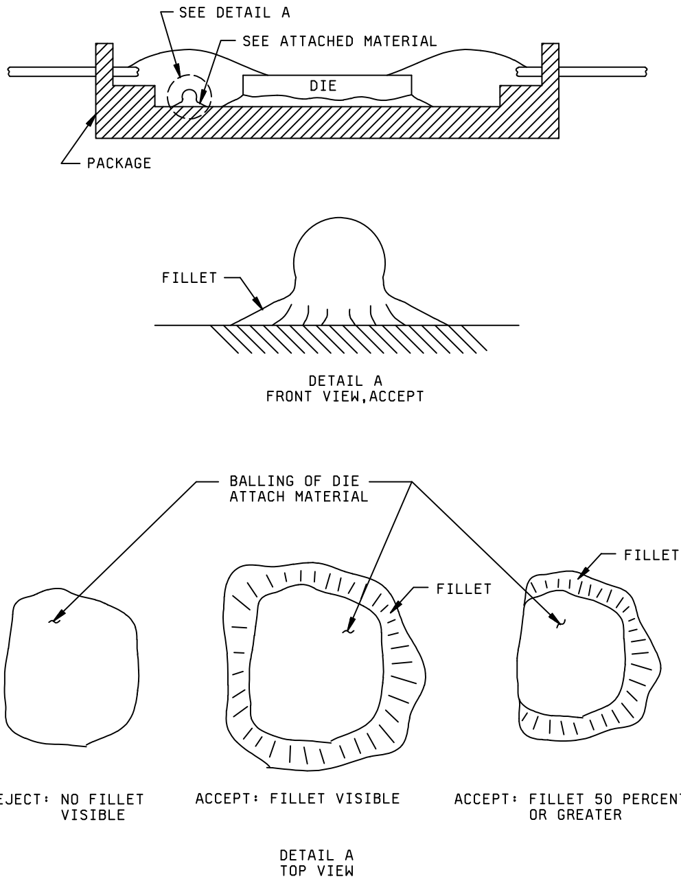
FIGURE 2010-36. Balling of die attach material.
